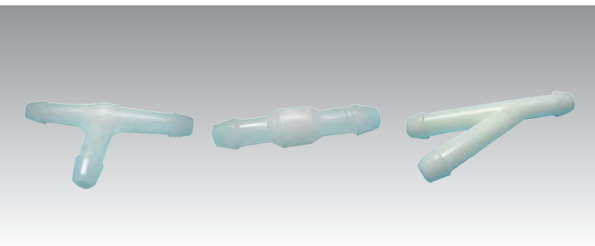
UTCL-203005F 2000/1.7/5.0/6.0 T CONNECTOR UTCL-200007 10000/1.7/8.0/9.0 I CONNECTOR UTCL-200006 10000/2.0/10/12 Y CONNECTOR
