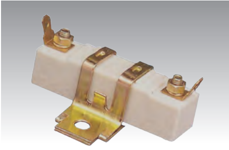
COIL RESISTOR 200/1.5/17/19 W/O WIRE P/N 22460-14606, 22460-14615 W WIRE P/N 90919-04027, 90919-04032
