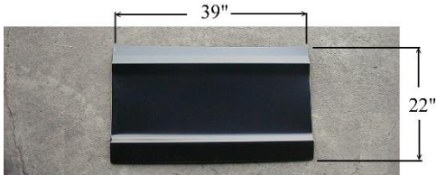
LG-10-006 FT. DOORSKIN HALF R/L FORD PICKUP 1967-72
