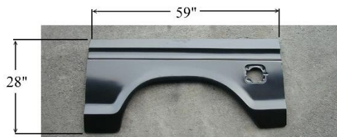
LG-10-031-6-A EXT. WHEEL ARCH – W/SQR HOLE LH FORD PICKUP 1973-79 & BRONCO 1978-79
