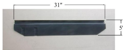
LG-TP-364 CAB FLOOR FOOTWELL SECTION, L=R FORD PICKUP 1980-91 (W/WEATHER STRIP CHANNEL)
