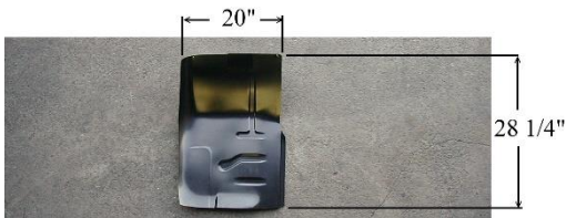
LG-TP-053/RH CAB FLOOR FT. SECTION RH FORD PICKUP 1980-98 & BRONCO 1980-96
