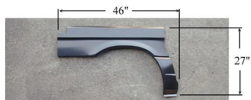
LG-TP-097/RH QUARTER PANEL LOWER SKIN RH AEROSTAR 1986-97 SHORT MODEL
