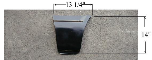
LG-10-045 L/RH QUARTER PANEL RR. LOWER L/RH ECONOLINE 1975-91 (124" WB)
