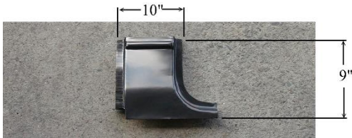
LG-10-008 L/RH LOWER DOOR POST REPAIR PANEL L/RH FORD PICKUP 1967-79 & BRONCO 1978-79
