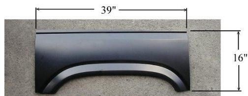
LG-10-035-6-4 L/RH UPPER WHEEL ARCH (39"x16") L/RH FORD PICKUP & BRONCO 1980-86
