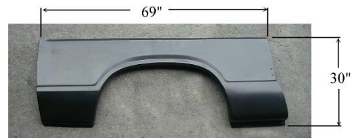
LG-10-016/RH QUARTER PANEL SKIN - W/HOLE RH ECONOLINE 1975-91
