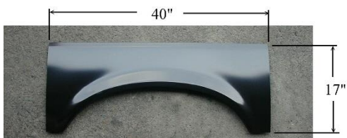
LG-TP-060 L/RH UPPER WHEEL ARCH (1.2MM) L/RH FORD PICKUP 1987-98 & BRONCO 1987-96
