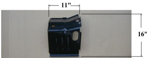
LG-10-744/RH CAB MOUNT PANEL RH FORD PICKUP & BRONCO 1980-86
