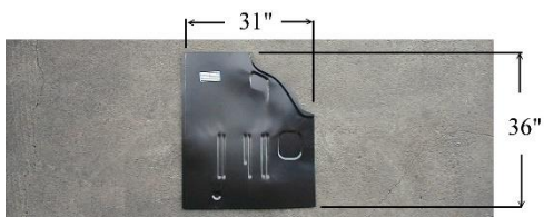
LG-10-042/LH CAB FLOOR RR. SECTION LH ECONOLINE 1975-91
