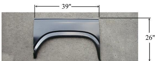
LG-10-035-6-3 L/RH UPPER WHEEL ARCH (39"x26") L/RH FORD PICKUP & BRONCO 1980-86
