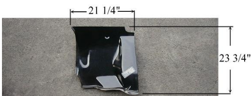
LG-10-041/LH CAB FLOOR FT. SECTION LH ECONOLINE 1975-91
