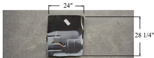
LG-TP-053/LH CAB FLOOR FT. SECTION LH FORD PICKUP 1980-98 & BRONCO 1980-96
