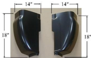
LG-TP-760 L/RH CAB CORNER L/RH (W 14" x H 18", 1.2MM) FD. P/U SUPERDUTY 1999-07 REGULAR CAB, CREW CAB
