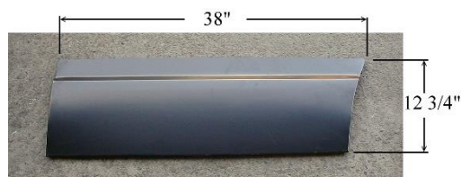
LG-TP-265 L/RH FT. DOORSKIN LOWER L/RH ECONOLINE 1975-91
