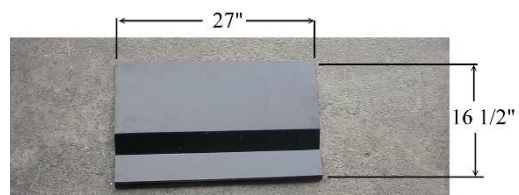
LG-TP-084 LARGE CAB CORNER EXT R/L FORD PICKUP 1980-98 SUPERCAB ONLY
