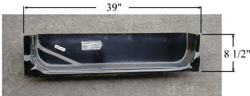
LG-10-007 L/RH INNER DOOR BOTTOM L/RH FORD PICKUP 1967-72
