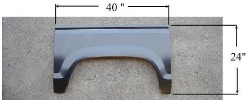
LG-10-061 L/RH EXT. WHEEL ARCH L/RH RANGER P/U 1983-88 ONLY
