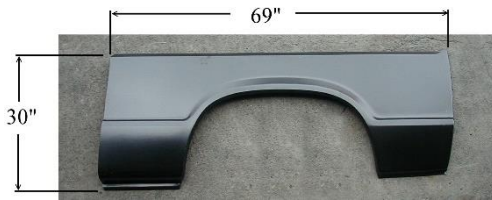
LG-10-016/LH QUARTER PANEL SKIN LH ECONOLINE 1975-91
